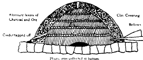
Fig. 86. Diagram of a bloomery hearth (after STRAKER, Wæalden Iron )
